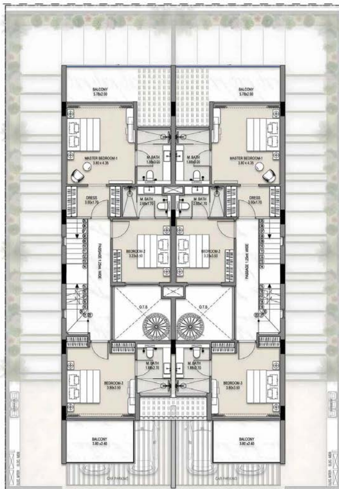
01 FIRST FLOOR PLAN SCALE 1:1000000
